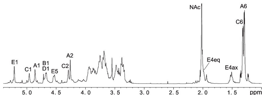
Figure 5. ^1\text{H} NMR spectrum of the OPS from Pseudomonas fluorescens BIM B-582. A–E refer to sugar units as shown in Table 2; NAc stands for the N -acetyl group.
