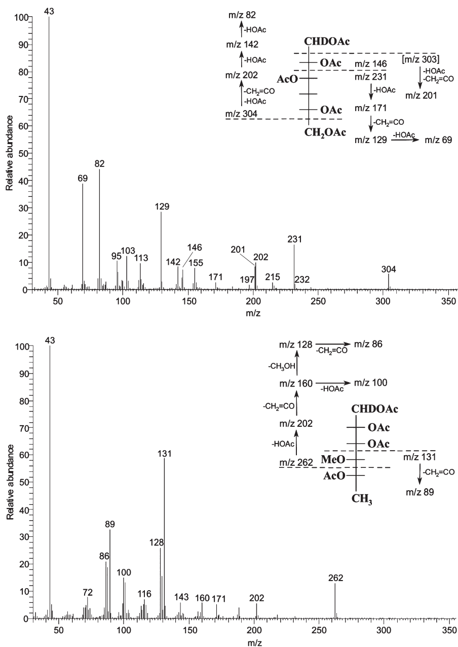
Figure 1. Electron impact mass spectra of 1,2,3,5,6-penta- O -acetyl-4-deoxyhexitol-1- d (top) and 1,2,3,5-tetra- O -acetyl-6-deoxy-4- O -methylhexitol-1- d (bottom). Structures and fragmentation pathways of the compounds are indicated in the insets. The putative parent ion with m/z 303 (indicated in square brackets) for the daughter ion with m/z 201 is evidently unstable and not seen in the spectrum of 1,2,3,5,6-penta- O -acetyl-4-deoxyhexitol-1- d .
