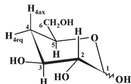
Figure 2. Structure of 4-deoxy-D-xyllo-hexose.
