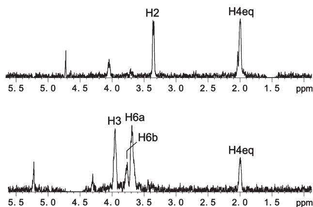
Figure 3. Parts of the one-dimensional ROESY spectra of the OPS from Pseudomonas fluorescens BIM B-582 with selective saturation of H-4ax at \delta_{\text{H}} 1.51 (top) and H-5 at \delta_{\text{H}} 4.53 (bottom) of 4dxylHex.
