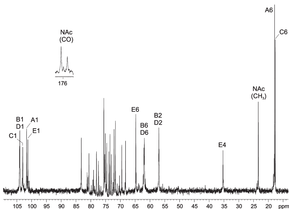
Figure 4. ^{13}\text{C} NMR spectrum of the OPS from Pseudomonas fluorescens BIM B-582. A–E refer to sugar units as shown in Table 2; NAc stands for the N -acetyl group.
